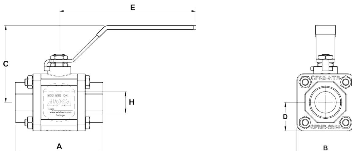
DIMENSIONS (mm)
