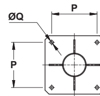
Pedestal base
