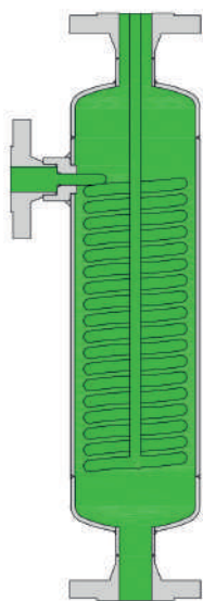
Fig. 1 - Cold system
