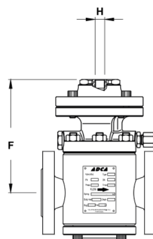
Fig. 3 - Dome loaded valve
